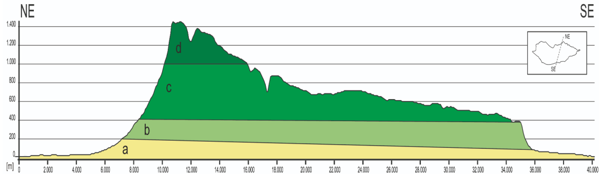
Figure 1. Section of the island of Soqatra along the dominant direction of the monsoon with the vegetation belts recognized by De Sanctis et al. (2012) (redrawn). a: Arid coastal plain; b: Transition zone; c: Arid limestone hills and plateaux; d: Semi-arid Haghier mountain.
