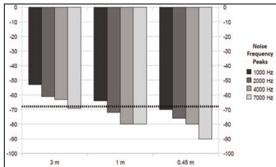
Figure 2. Effect of cable length in the mitigation of Ultrasonic 250 inherent noise. Vertical axis: sound pressure (dB), horizontal axis: USB cable length (m), dashed line: typical Ultrasonic 250 noise floor under ideal field recording conditions (-68 dB ref full scale level).
