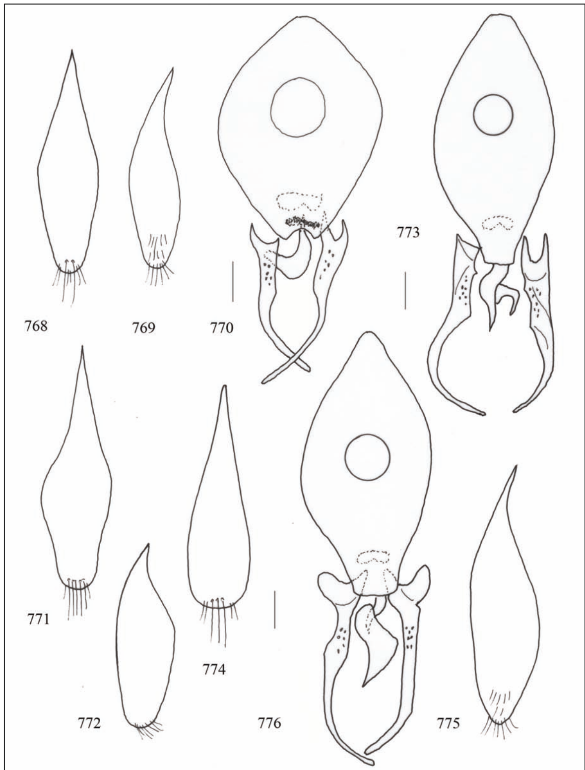
Figures 768–776. Tergite and sternite of the male genital segment, aedeagus of Notolinopsis submontanus n. sp. (Figs. 768–770). Tergite and sternite of the male genital segment, aedeagus of Notolinopsis uncinatus n. sp. (Figs. 771–773). Tergite and sternite of the male genital segment, aedeagus of Notolinopsis lungweianus n. sp. (bar scale: 0.1 mm) (Figs. 774–776).
