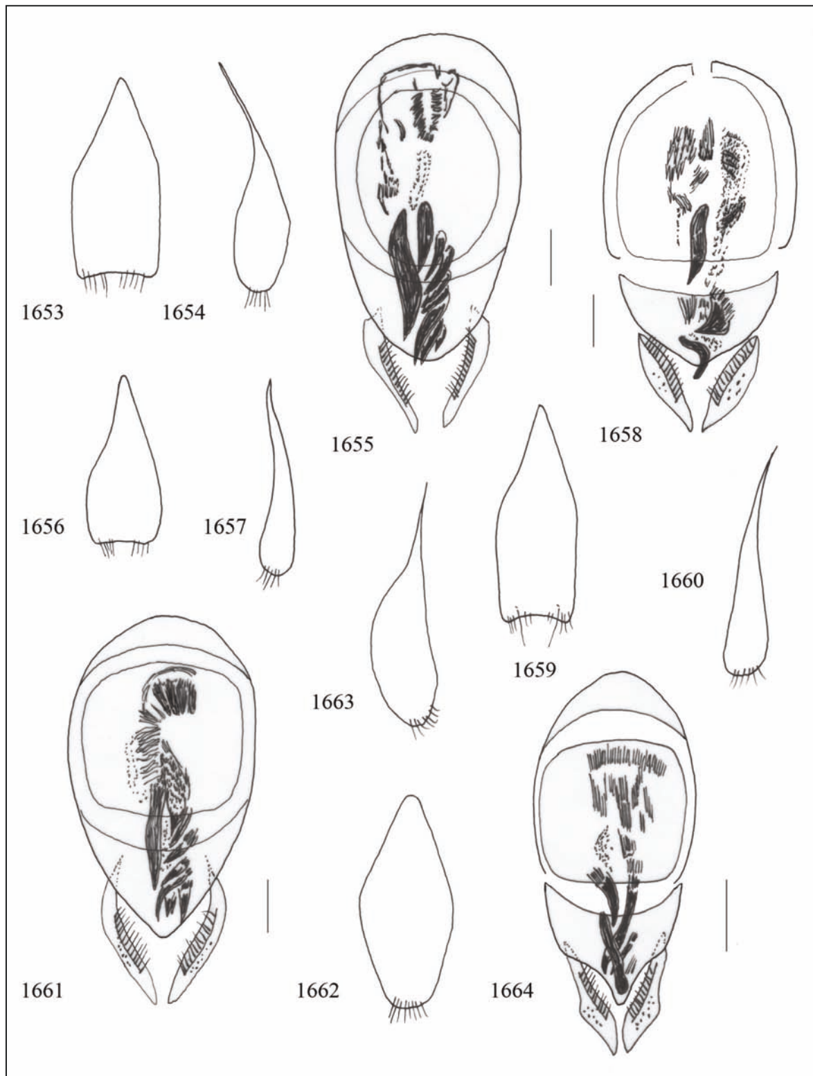
Figures 1653–1664. Tergite and sternite of the male genital segment, aedeagus of Chaetocinus anommatophilus (Figs. 1653–1655), C. sibiensis n. sp. (Figs. 1656–1658), C. dorylophilus n. sp. (Figs. 1659–1661), and C. guineanus n. sp. (Figs. 1662–1664) (bar scale: 0.1 mm).
