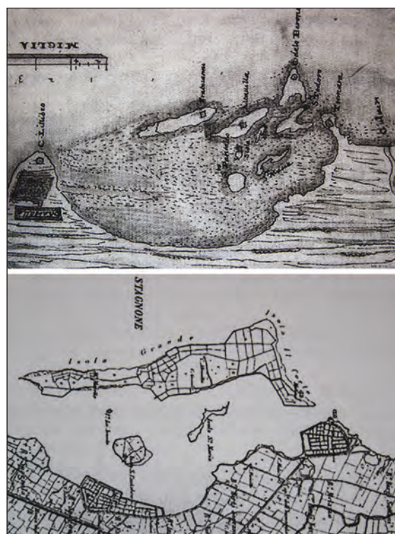
Figures 31, 32. The islands (above) that formed the Isola Lunga of Marsala (below): “the island that was not there” according to Donato (2013; see also Spannocchi, 1596 and Dufour, 1992).
