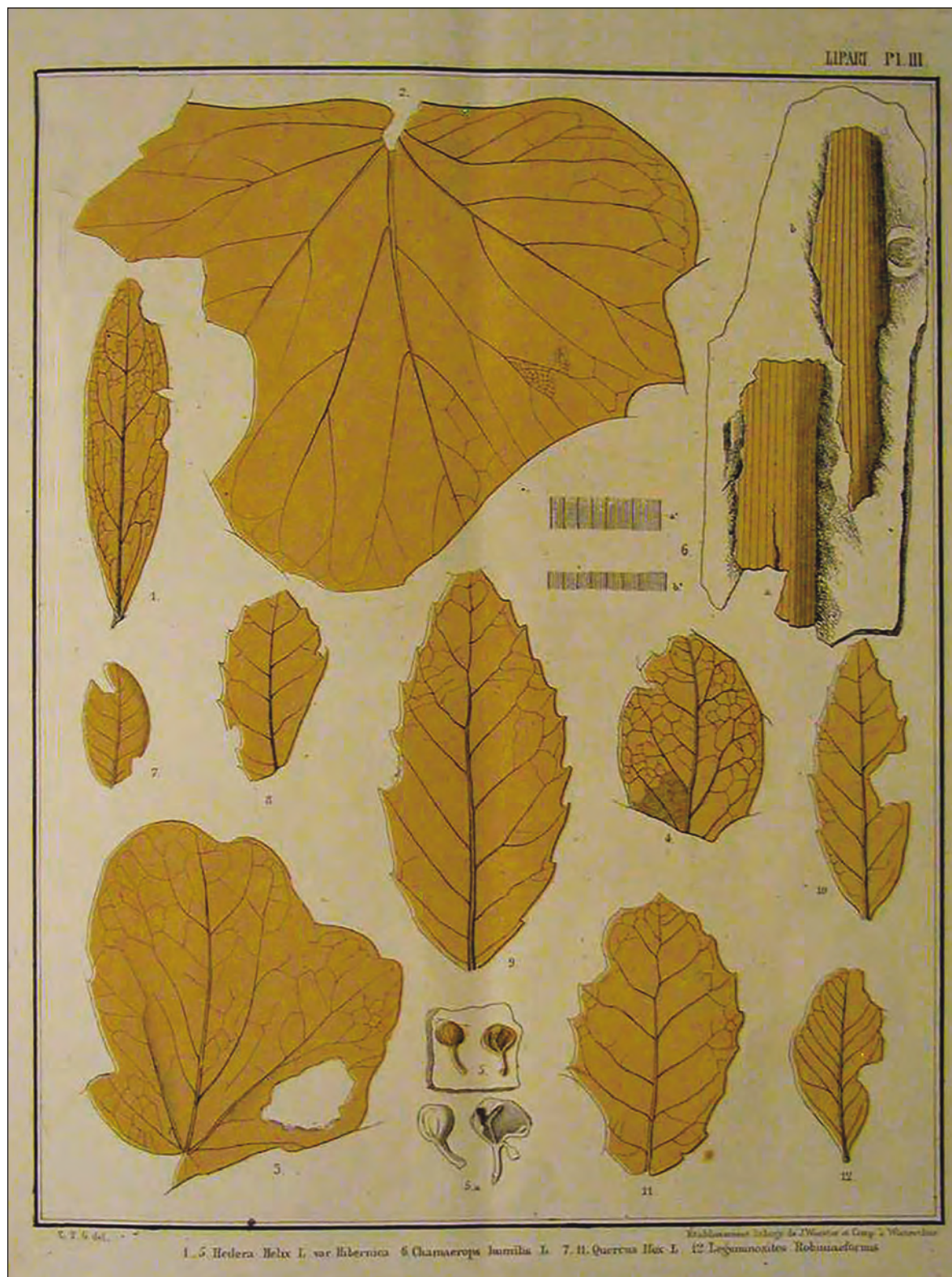
Figure 67. Volcanic tuffs and siliceous limestones of Lipari by Gaudin & Pirajno (1860), plate 3: the drawings show some leaves of Hedera helix L. figures 1–5), Chamaerops humilis L. (figure 6), leaves of Quercus ilex L. (figures 7–11) and a plant “Robiniaeformis”, Leguminosae (figure 12).
